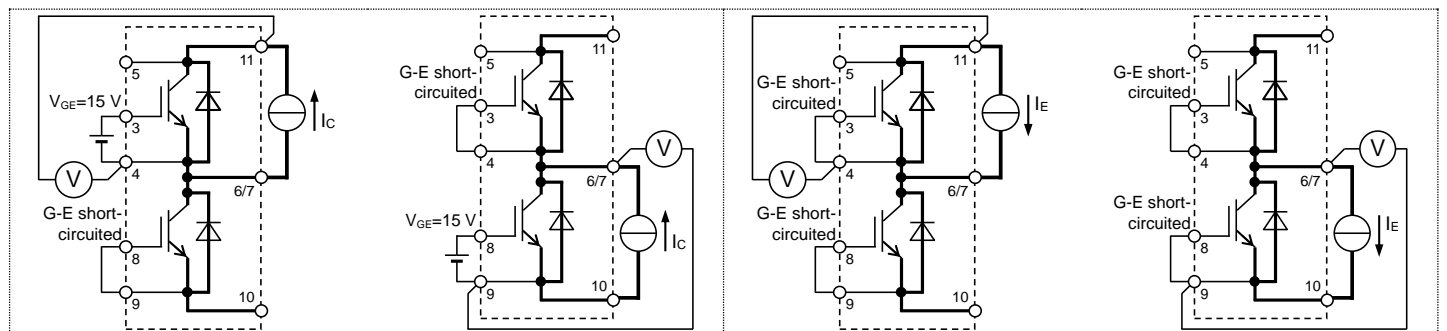
V_{EC} characteristics test circuit
